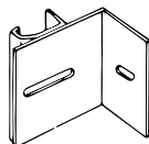
Angle Mounted Track Continuous leg-out angle used on larger doors to attach to wood jambs
